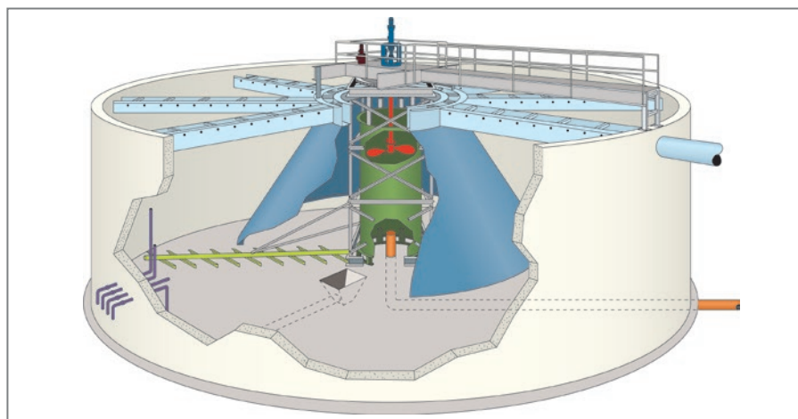
Cutaway diagram of the CONTRAFLO Solids Contact Clarifier
